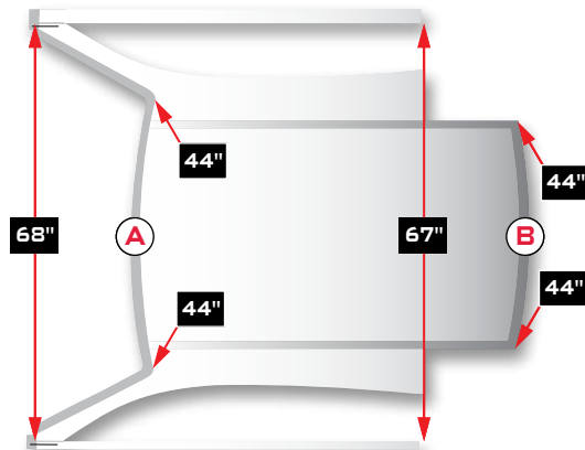
TRADITIONAL ROOF
