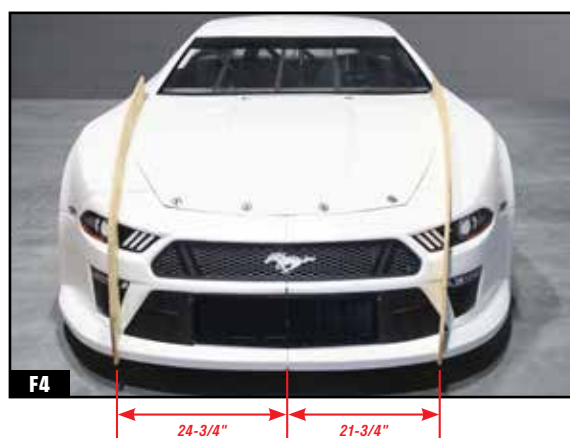
BOTH FENDER TEMPLATES ARE LOCATED AT THE INTERSECTION OF THE FENDER AND HOOD AT THE REAR OF THE TEMPLATE.
