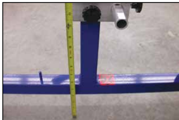
ADJUST BLOCK SO TREAD WIDTH GAUGE IS LOCATED TO CENTER OF WHEEL (APPROXIMATELY 12-½ INCHES UP FROM GROUND). THIS DIMENSION WILL VARY BASED ON TIRE SIZE.
