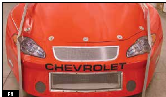
LEFT SIDE TEMPLATE IS LOCATED 23-7/8 INCHES FROM CENTERLINE. RIGHT SIDE TEMPLATE IS LOCATED 26 INCHES FROM CENTERLINE.
