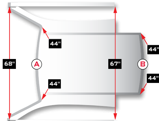
TRADITIONAL ROOF
