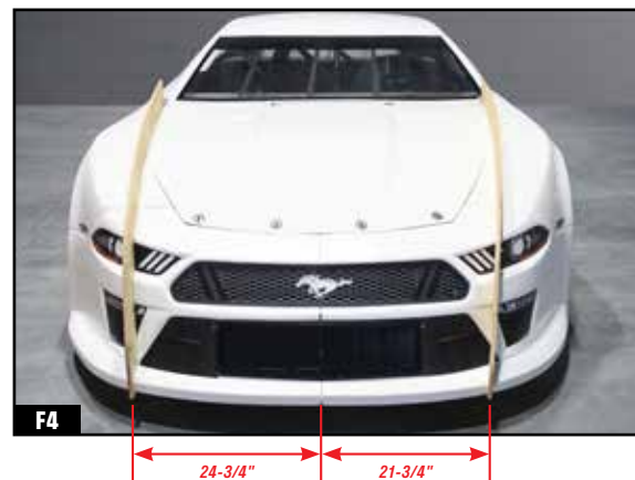
BOTH FENDER TEMPLATES ARE LOCATED AT THE INTERSECTION OF THE FENDER AND HOOD AT THE REAR OF THE TEMPLATE.
